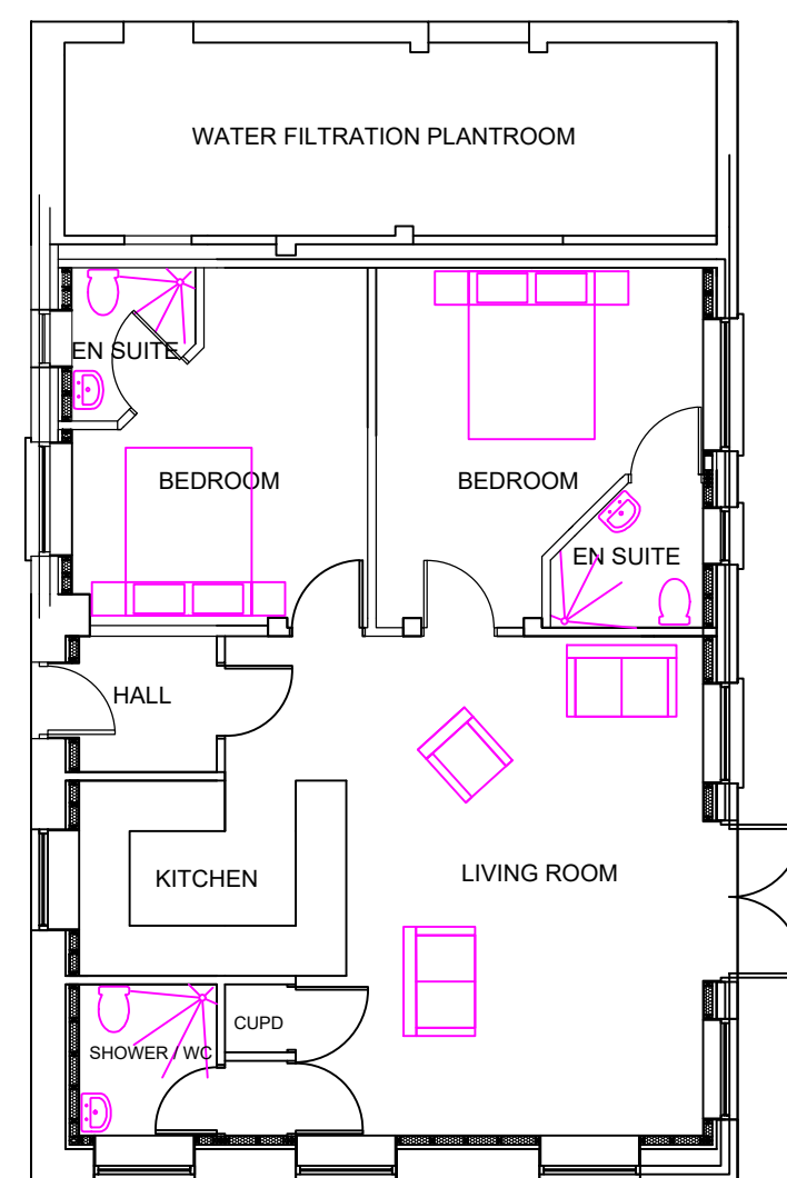
PROPOSED GF PLAN OPTION 4
