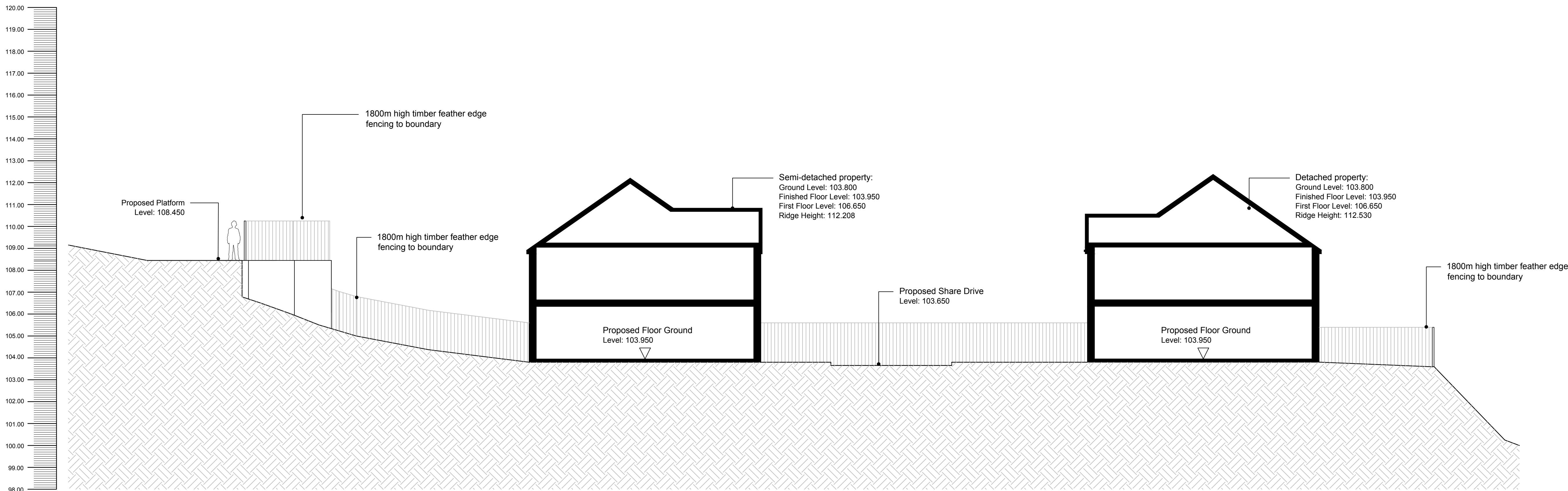
PROPOSED SECTION A-A SCALE 1:100 @ A1
