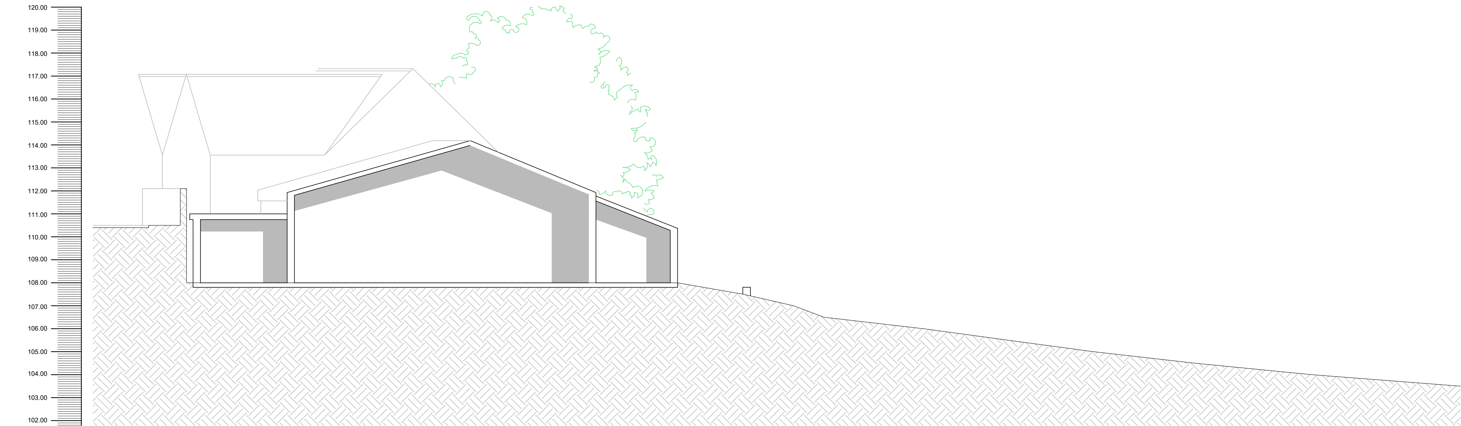
EXISTING SECTION B-B SCALE 1:100 @ A1
