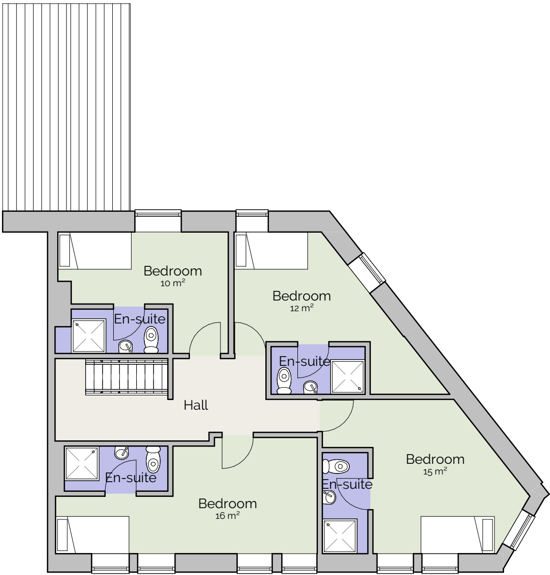
2 First Floor 1 : 100
