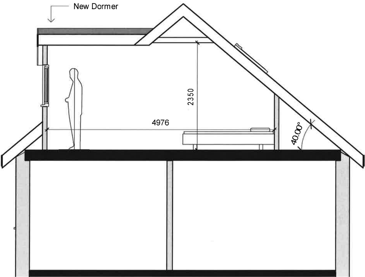
Proposed Section 2 1 : 50
