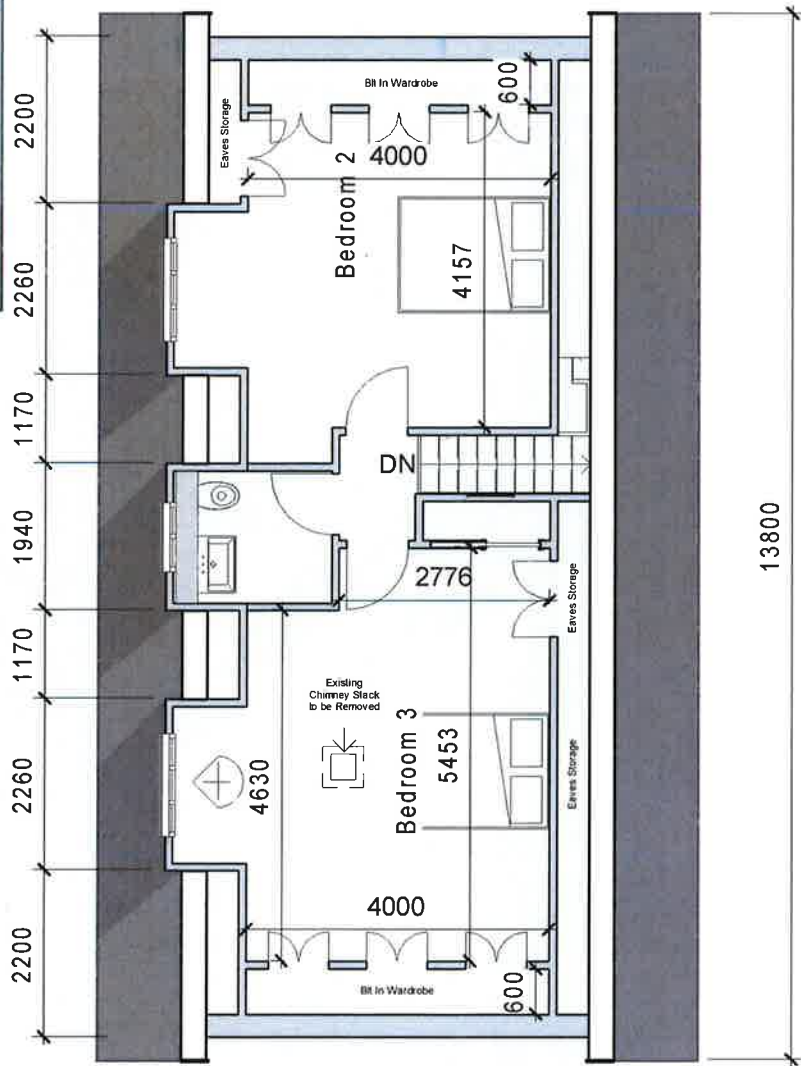
Example Gable End Built in Wardrobes
