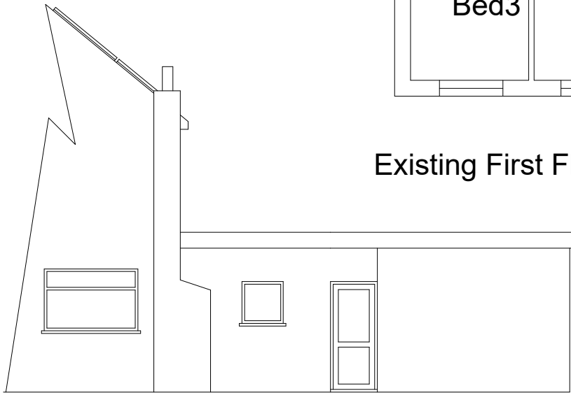
Existing Side Elevation Facing No4
