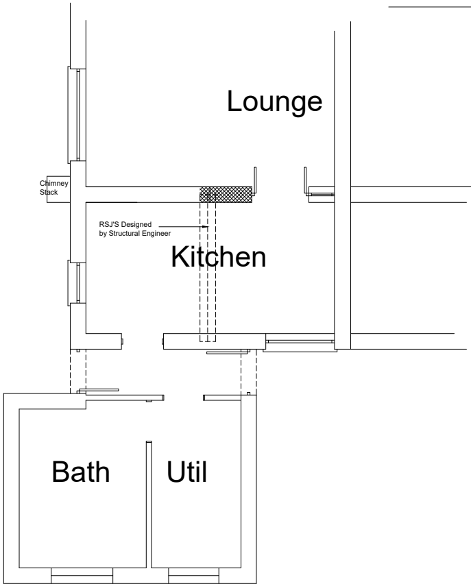
Proposed Ground Floor Layout
