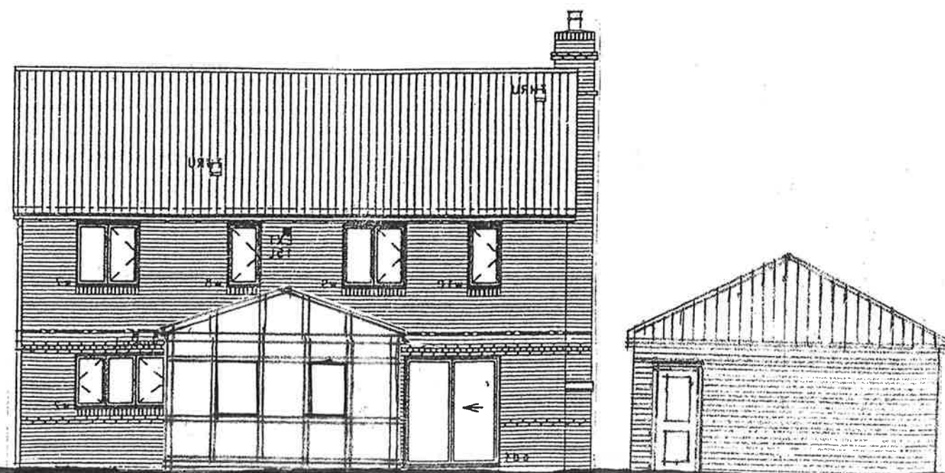
SIDE ELEVATION
