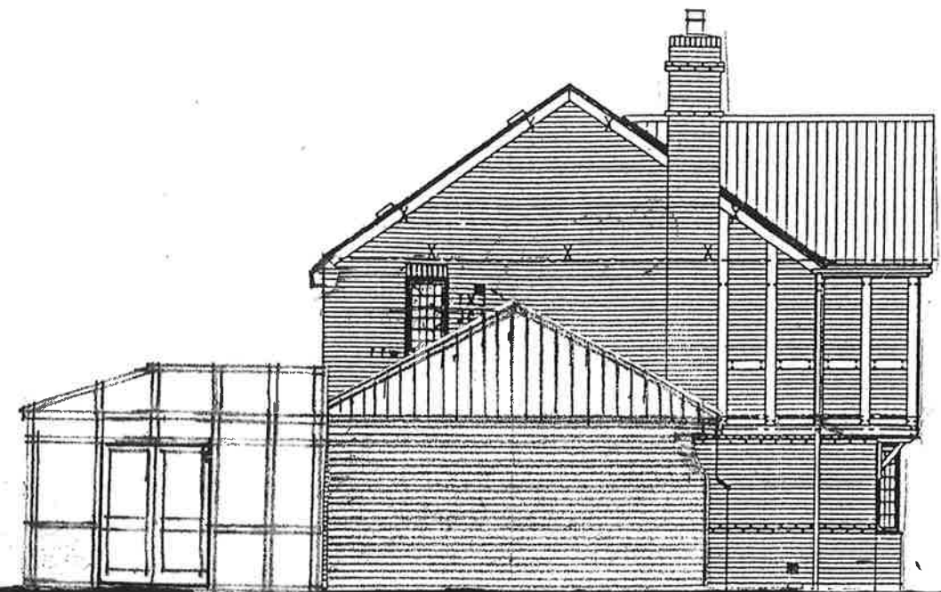
REAR ELEVATION
