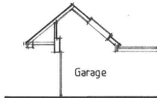
CROSS SECTION
