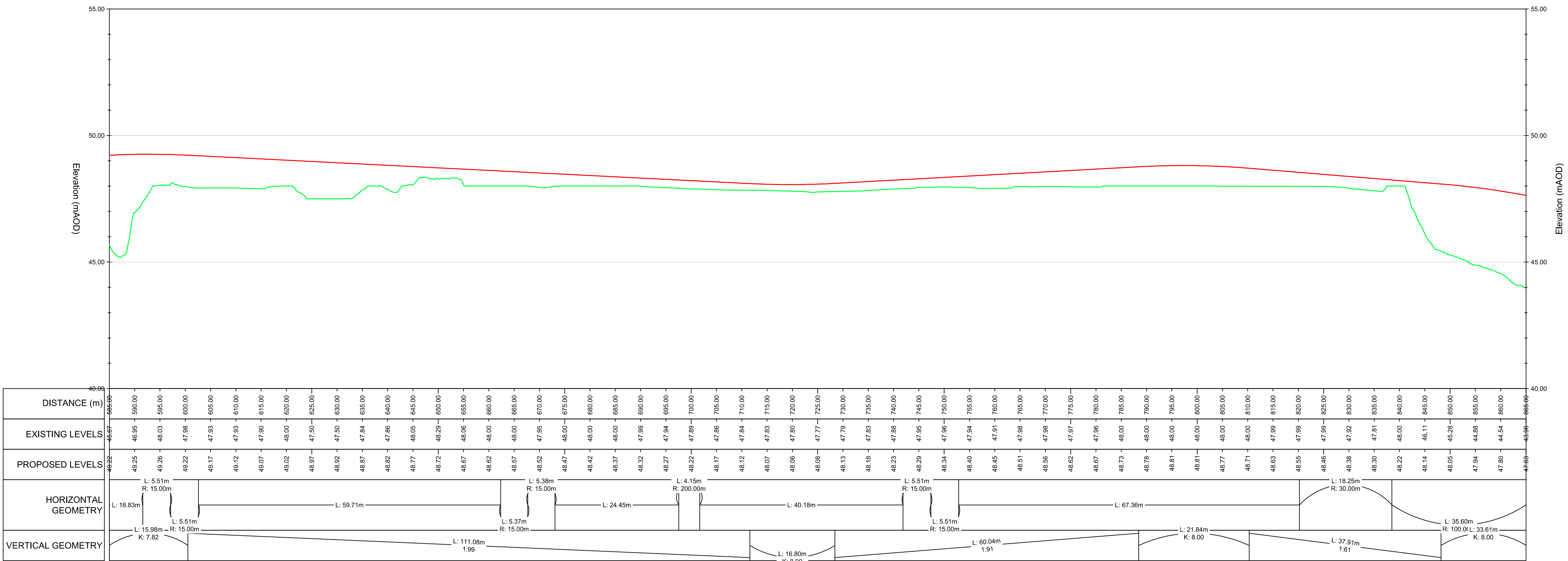
Section Alignment - ROAD 1 - Centreline - Alignment - ROAD 1 - Centreline (Vertical Exaggeration x5.00)
