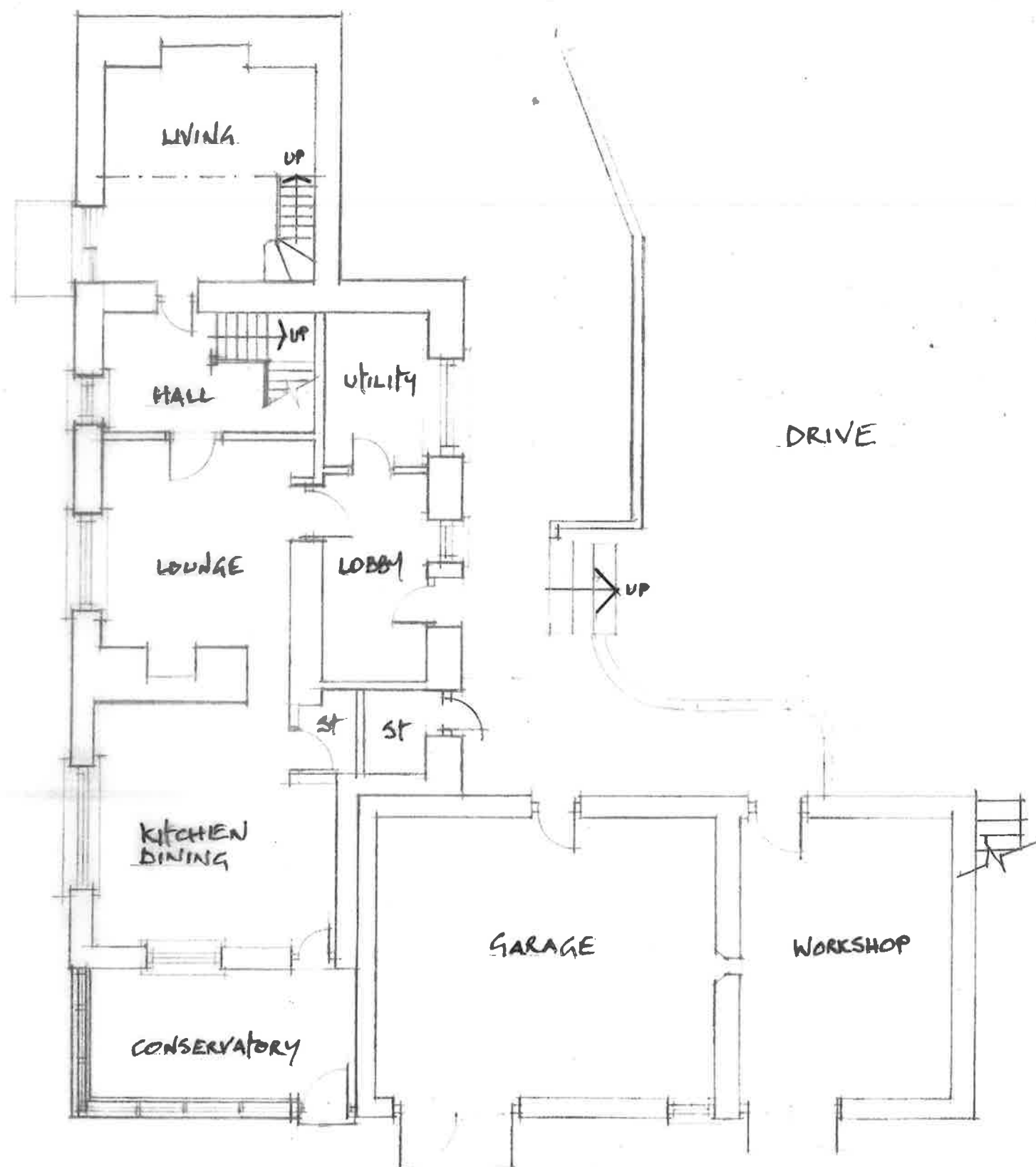
GROUND FLOOR
