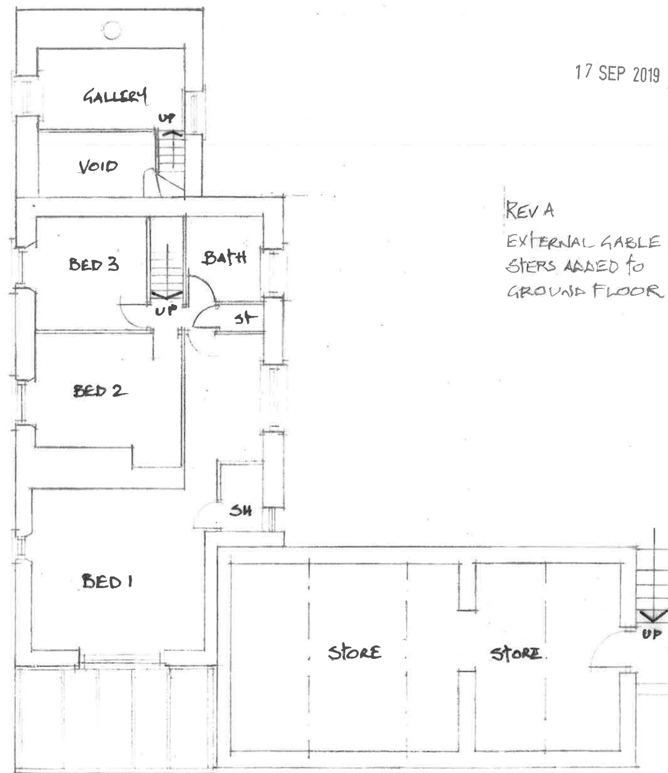
FIRST FLOOR
