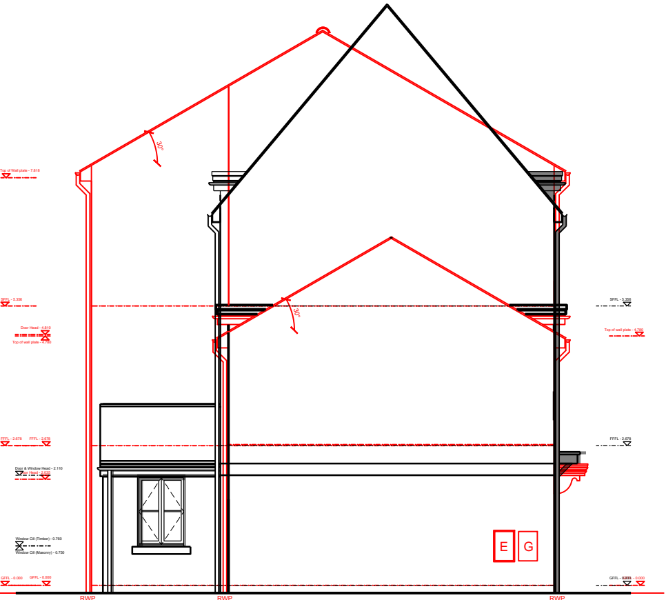
SIDE ELEVATION 2
