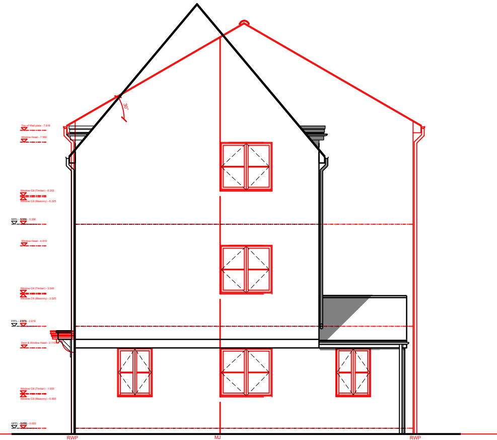
SIDE ELEVATION 1
