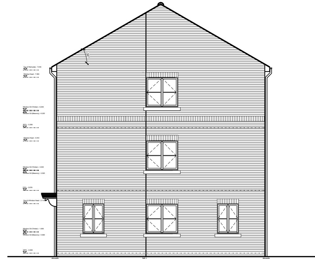
SIDE ELEVATION 1
