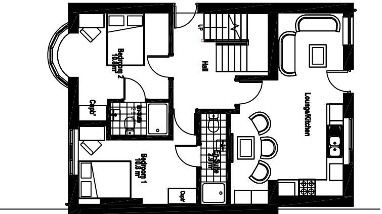
Proposed Ground Floor Plan Scale: 1 : 100
