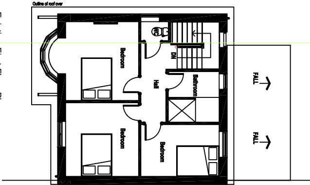
Existing First Floor Plan Scale: 1 : 100
