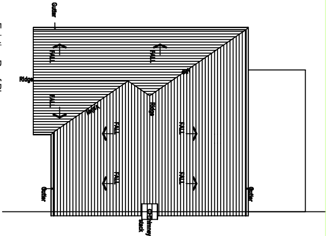
Existing Roof Plan Scale: 1 : 100
