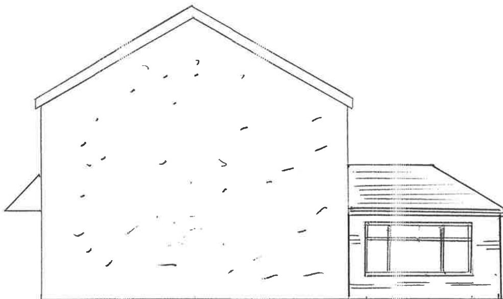
PROPOSED PINE END ELEVATION
