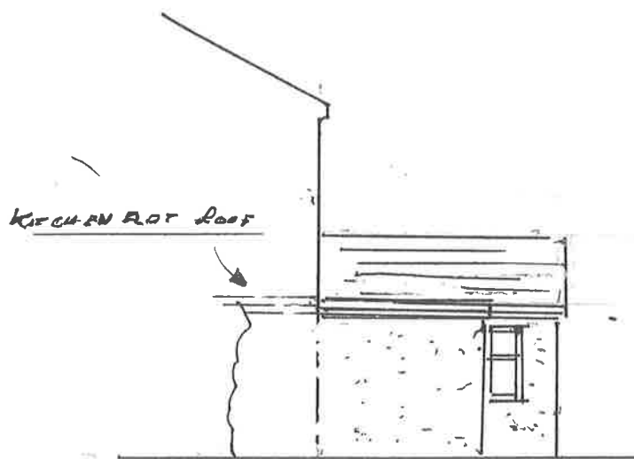
PROPOSED RH SIDE ELEVATION
