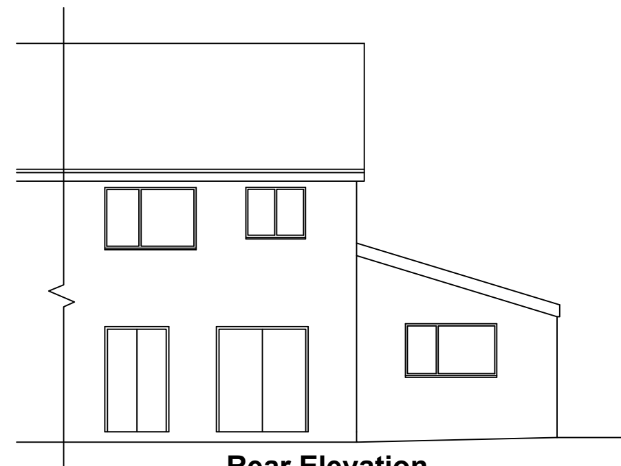
Rear Elevation
