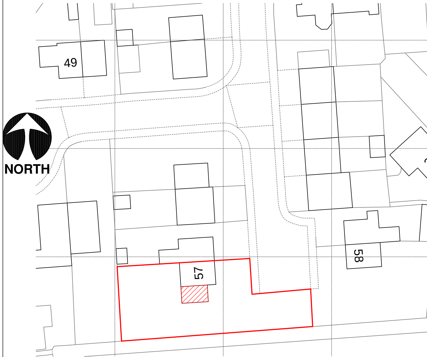
Block Plan 1-500
