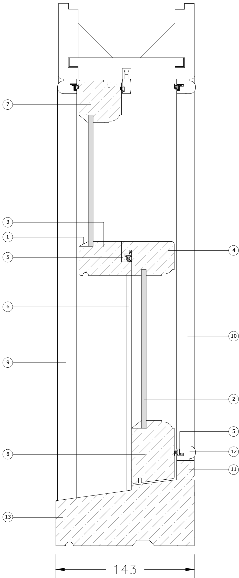
PROPOSED SECTION DETAIL SCALE 1:2 @ A3
