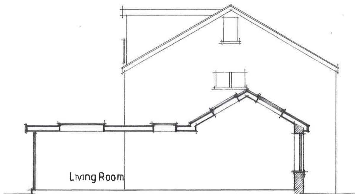
CROSS SECTION (1:100)
