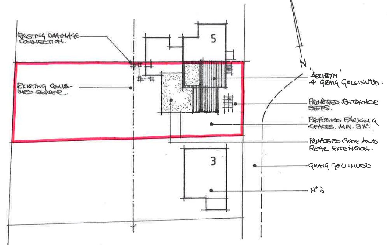
BLOCK PLAN 1:500
