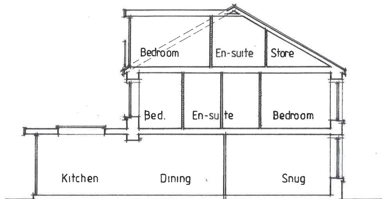
CROSS SECTION (1:100)
