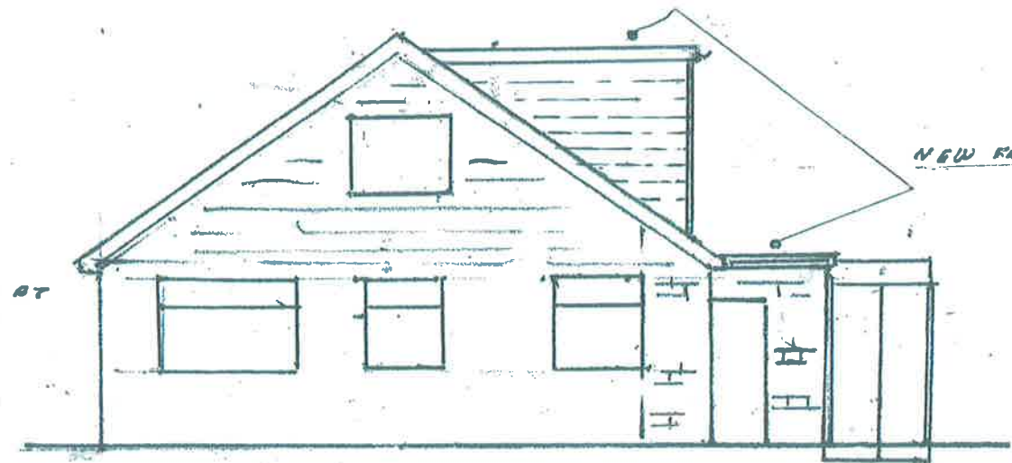
PROPOSED FRONT ELEVATION FACING ROAD
