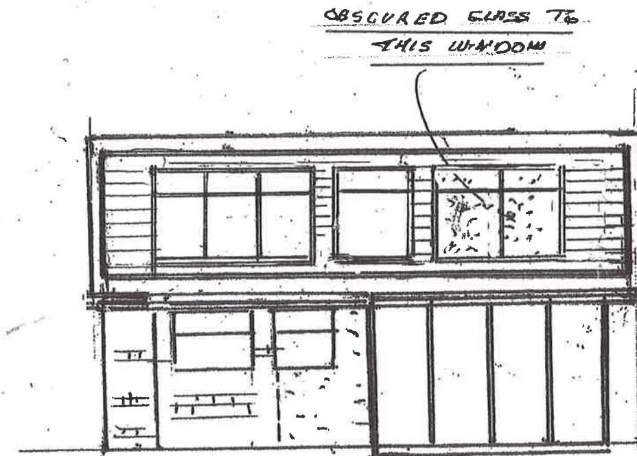
PROPOSED RH SIDE ELEVATION
