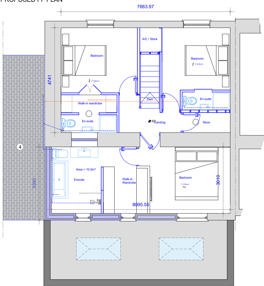
PROPOSED FF PLAN
