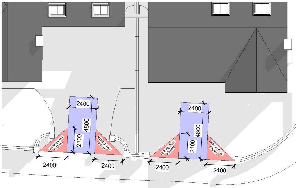
1 Visibility Splays 1 : 200
