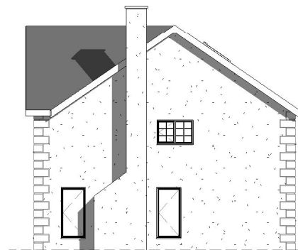
6 Plot 2 - Right Elevation 1 : 200
