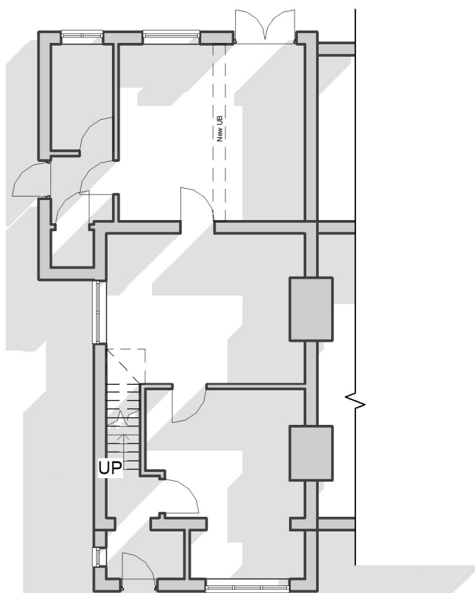
3 00 Ground Floor - Proposed 1 : 125
