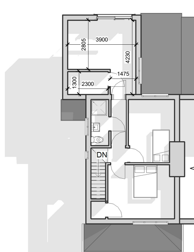
4 01 First Floor - Proposed 1 : 125
