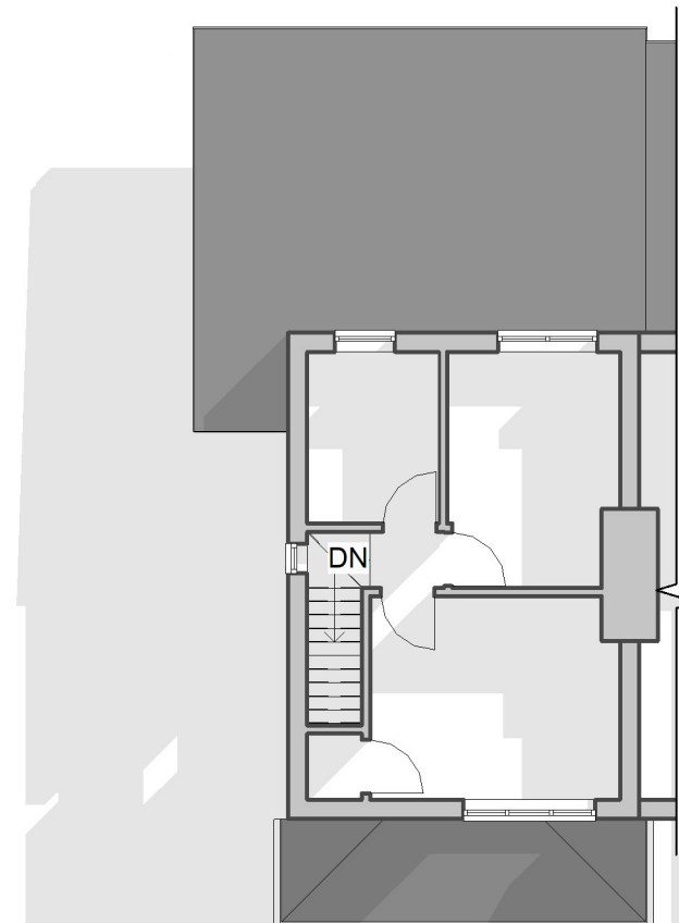
2 01 First Floor - Existing 1 : 125
