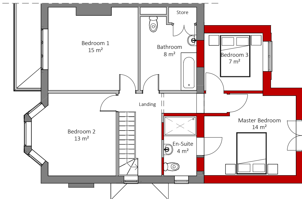
First Floor
