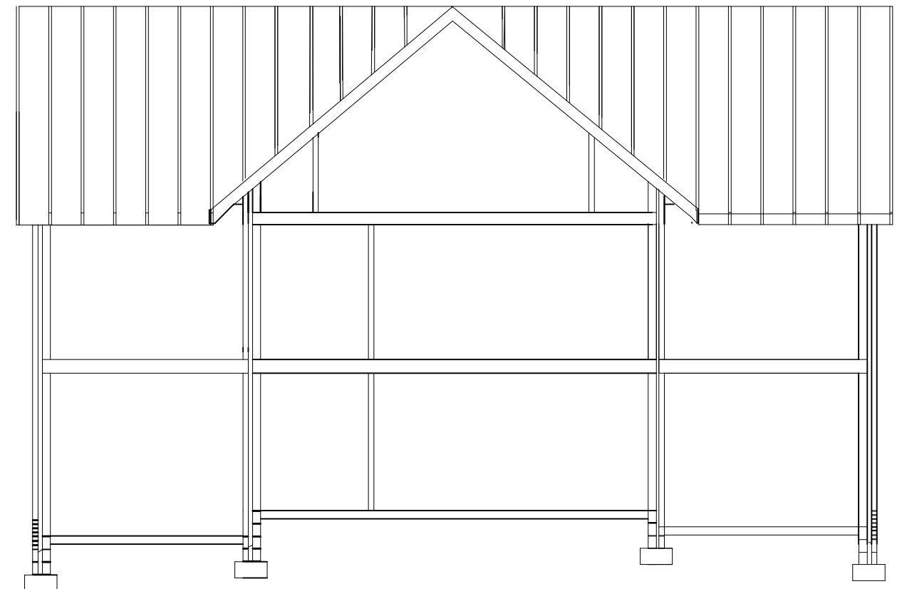
Front Section Scale 1:100
