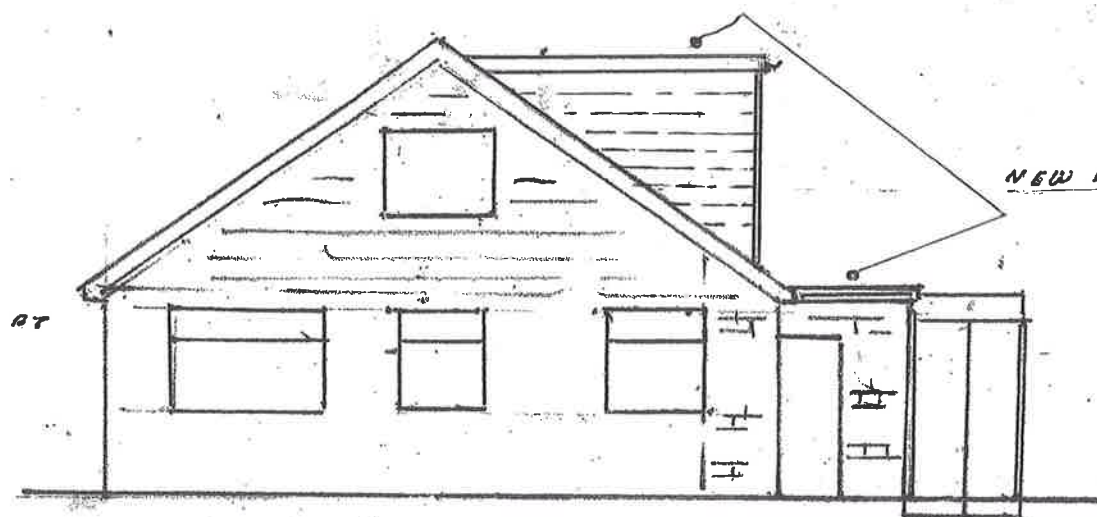
PROPOSED FRONT ELEVATION FACING ROAD
