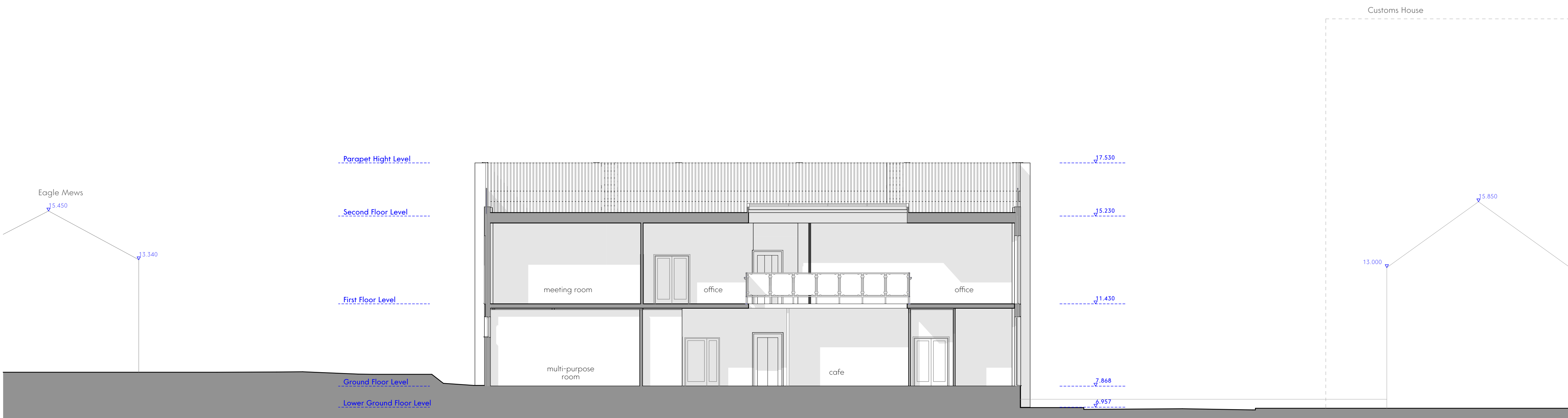
Proposed Section 03
