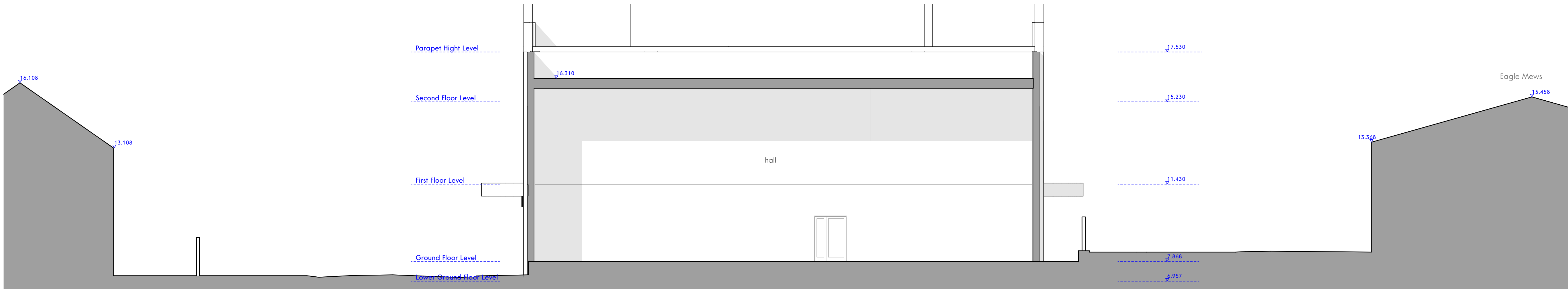
Proposed Section 04
