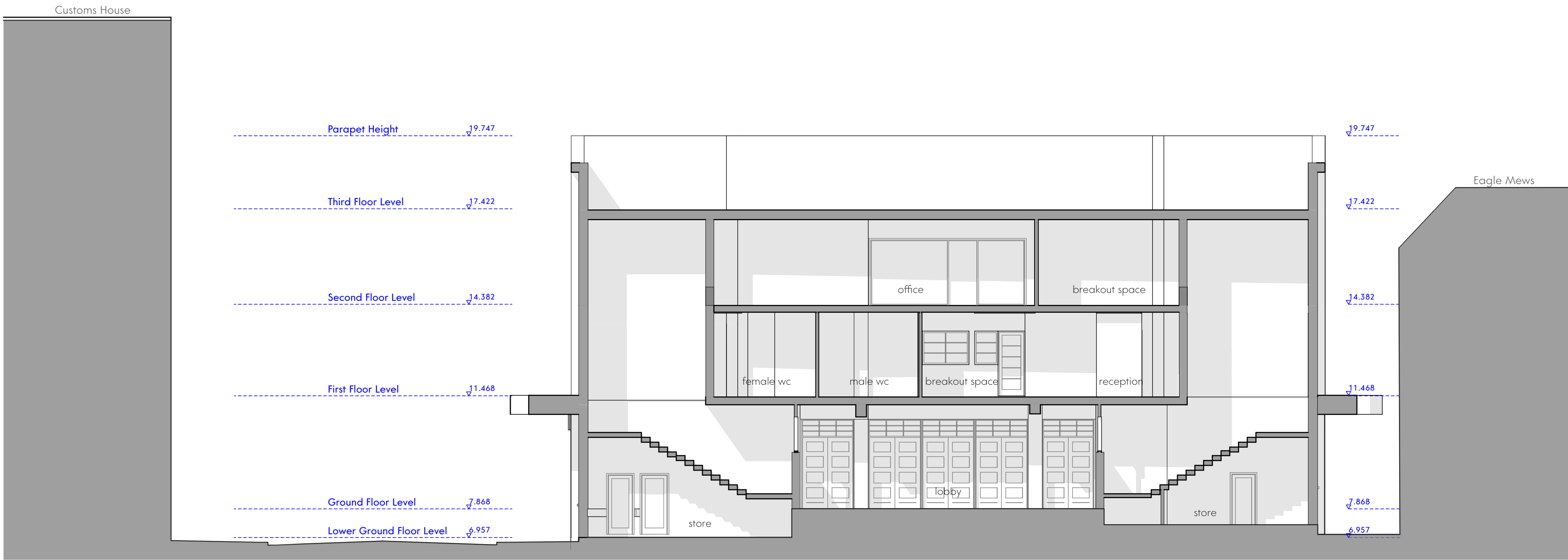
Proposed Section 02
