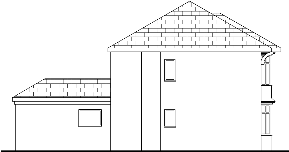
Side Elevation on B
