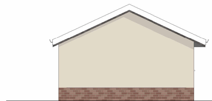
5 Proposed Outbuilding Side Elevation (2) 1 : 100
