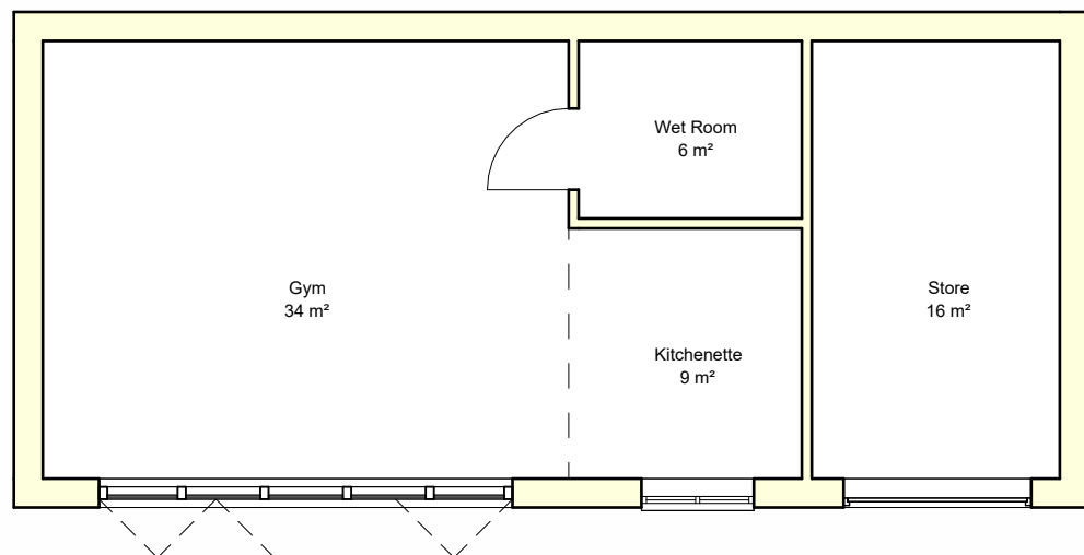
1 1.2 - Proposed Outbuilding Plan 1 : 100
