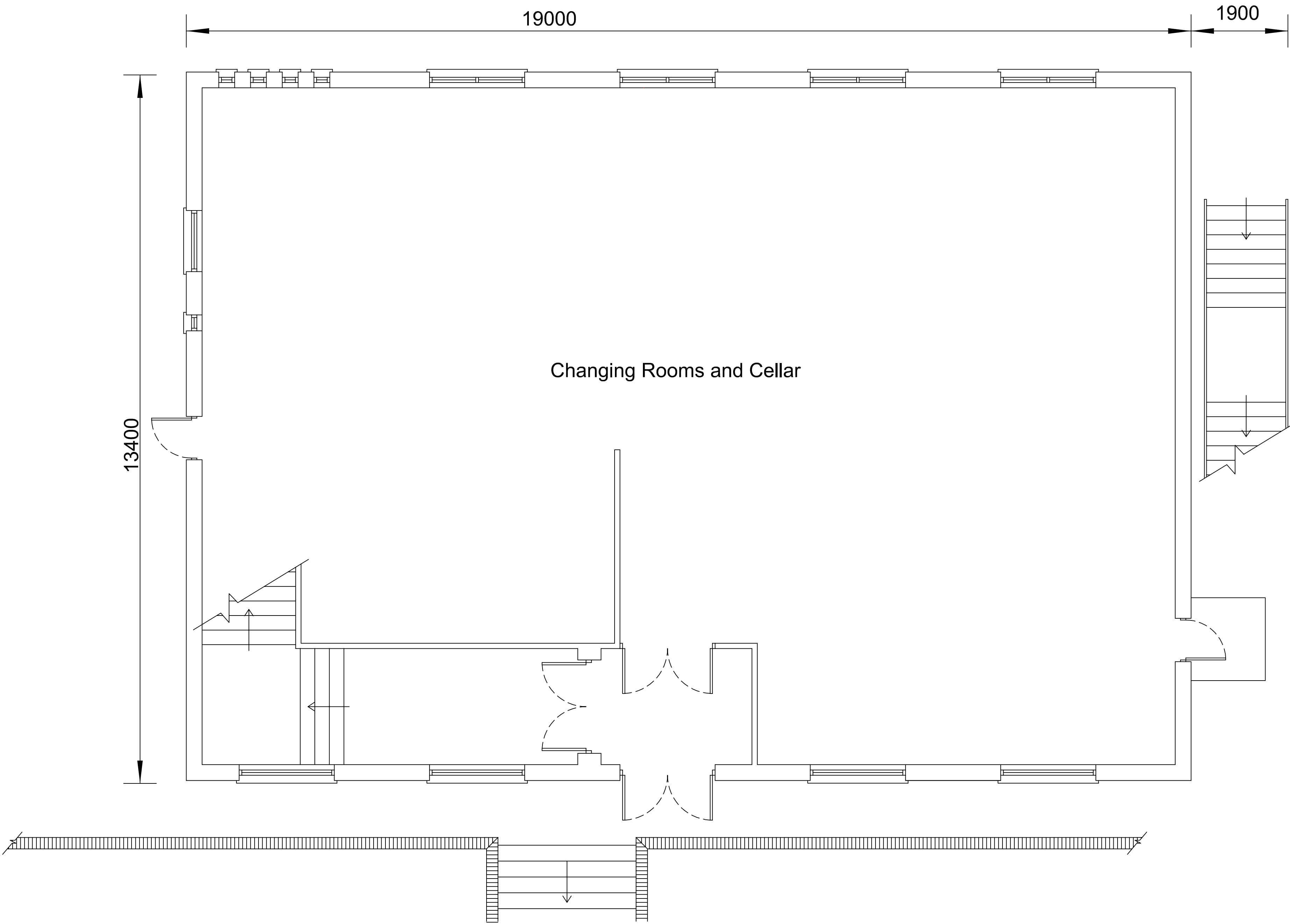
Existing Ground Floor
