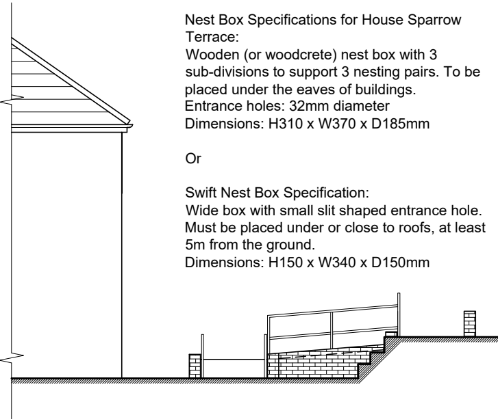
Proposed Side Serction / Elevation
