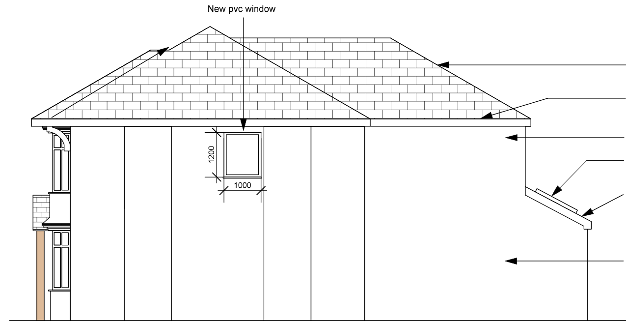
Side Elevation on B
